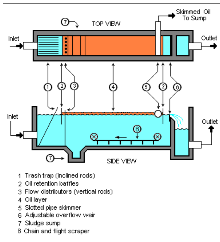
Figure 26: Typical API oil separator (Source: API, 1990)
