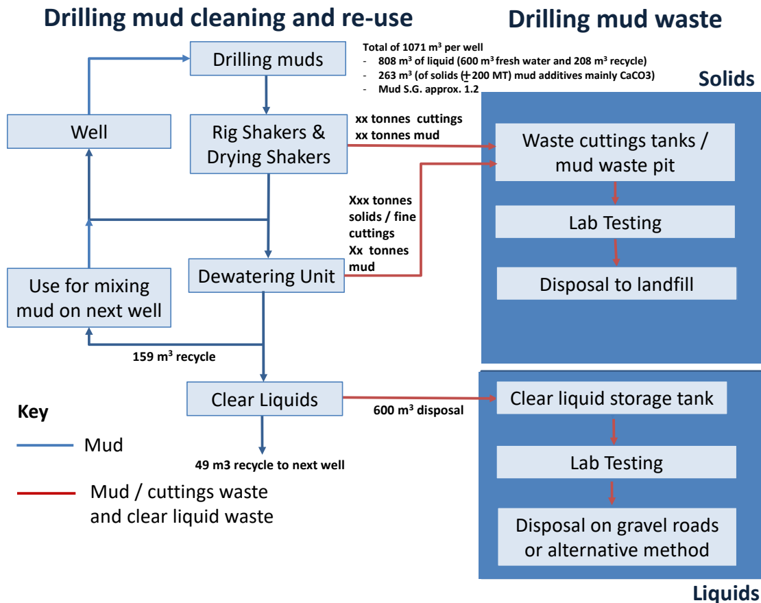
Figure 14: Process for the Generation of Drilling Waste
