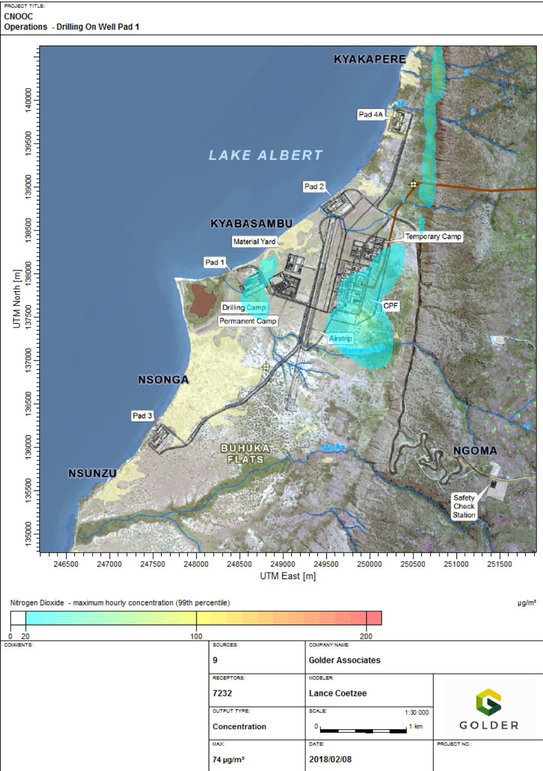
Figure 47: Operations - drilling on well pad 1, \text{NO}_2 maximum hourly concentration (99 th percentile).
