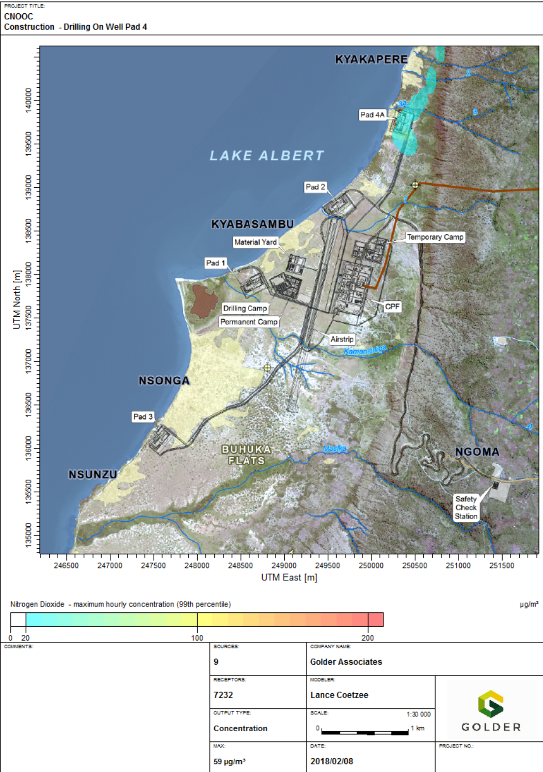
Figure 42: Construction - drilling on well pad 4, NO 2 maximum hourly concentration (99 th percentile).
