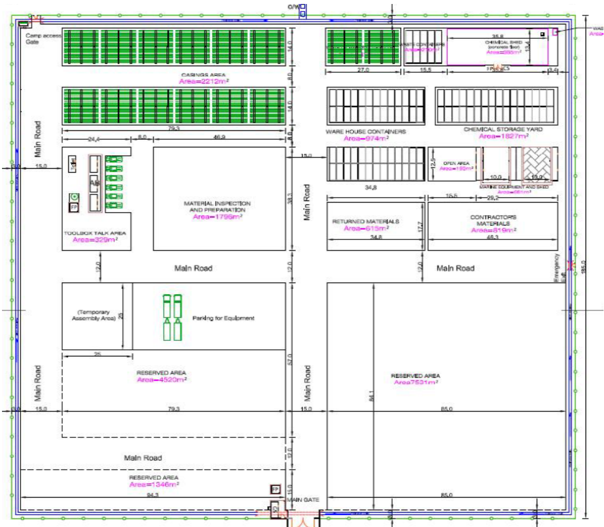
Figure 33: Layout for a typical materials yard.
