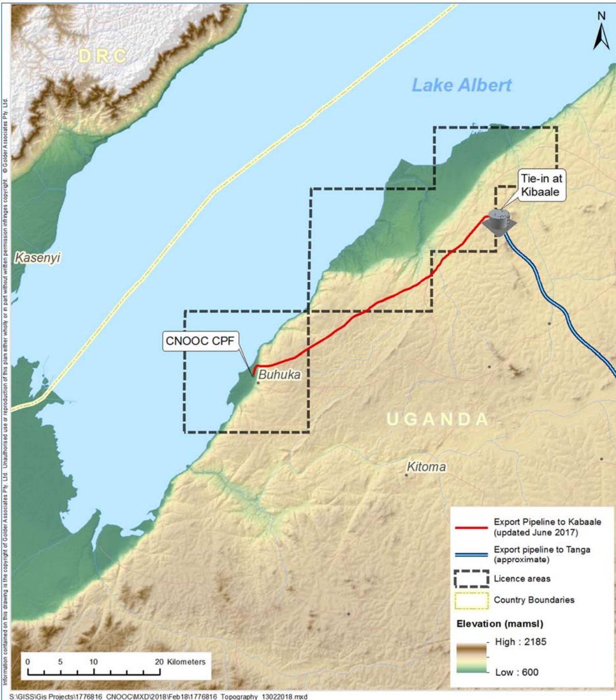
Figure 31: Location of the export pipeline
