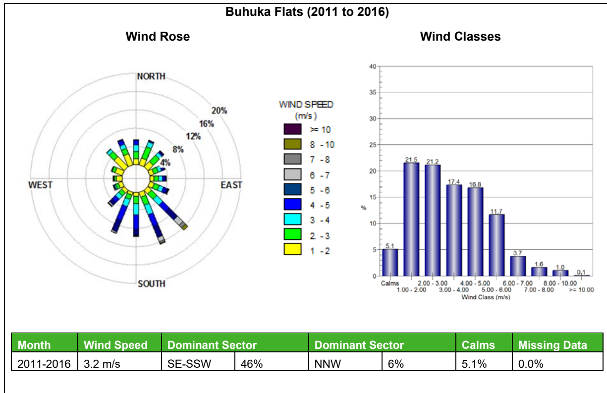
Figure 20: Period Wind Rose – Buhuka Flats 2011 - 2016.
