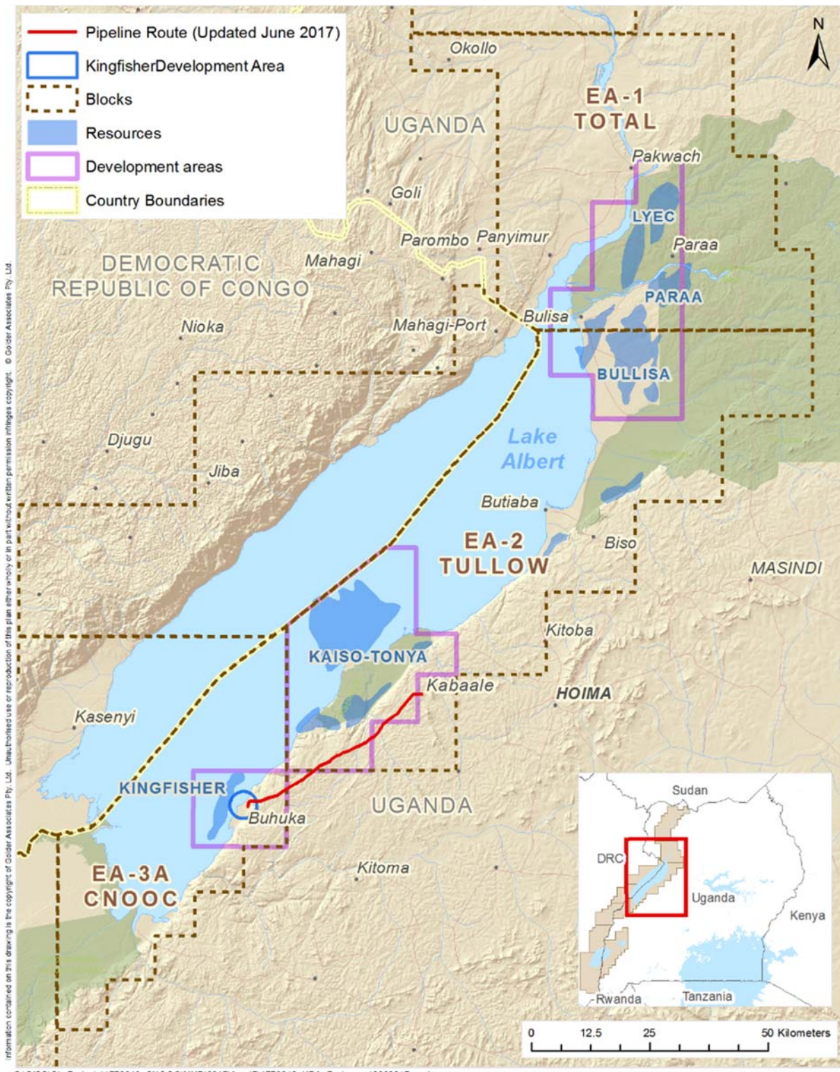
Figure 1: Kingfisher Development Area
