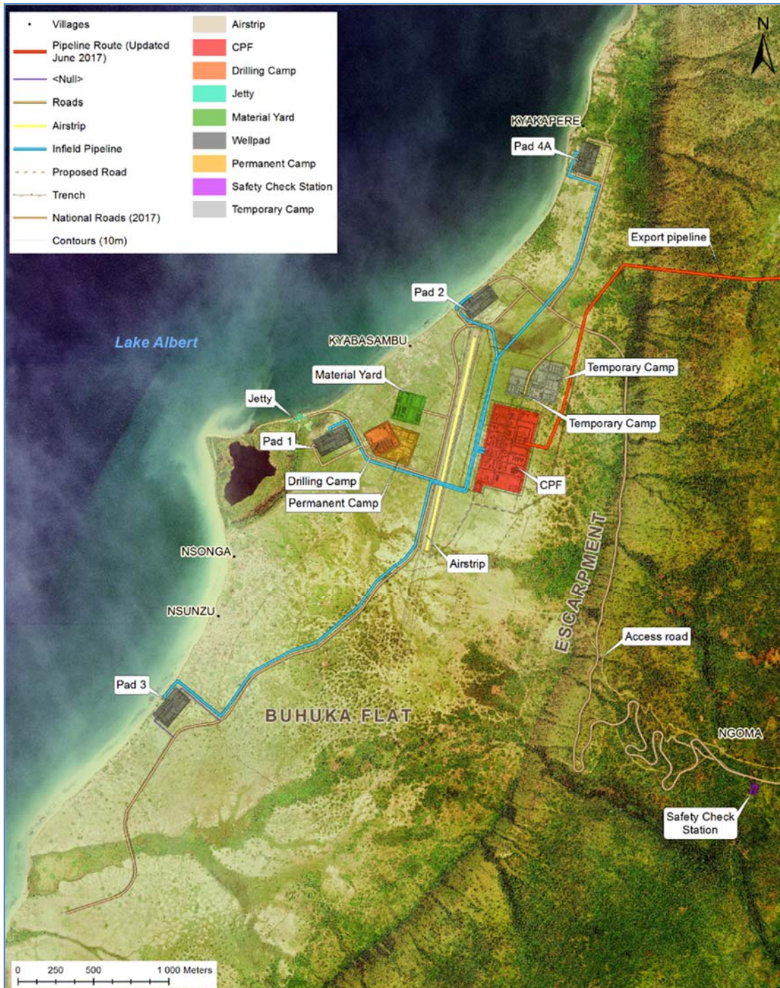
Figure 3: Project infrastructure
