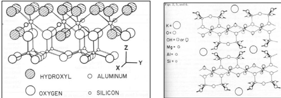
Figure 6: 1:1 and 2:1 clay mineralogy (fraction <0,002mm)
