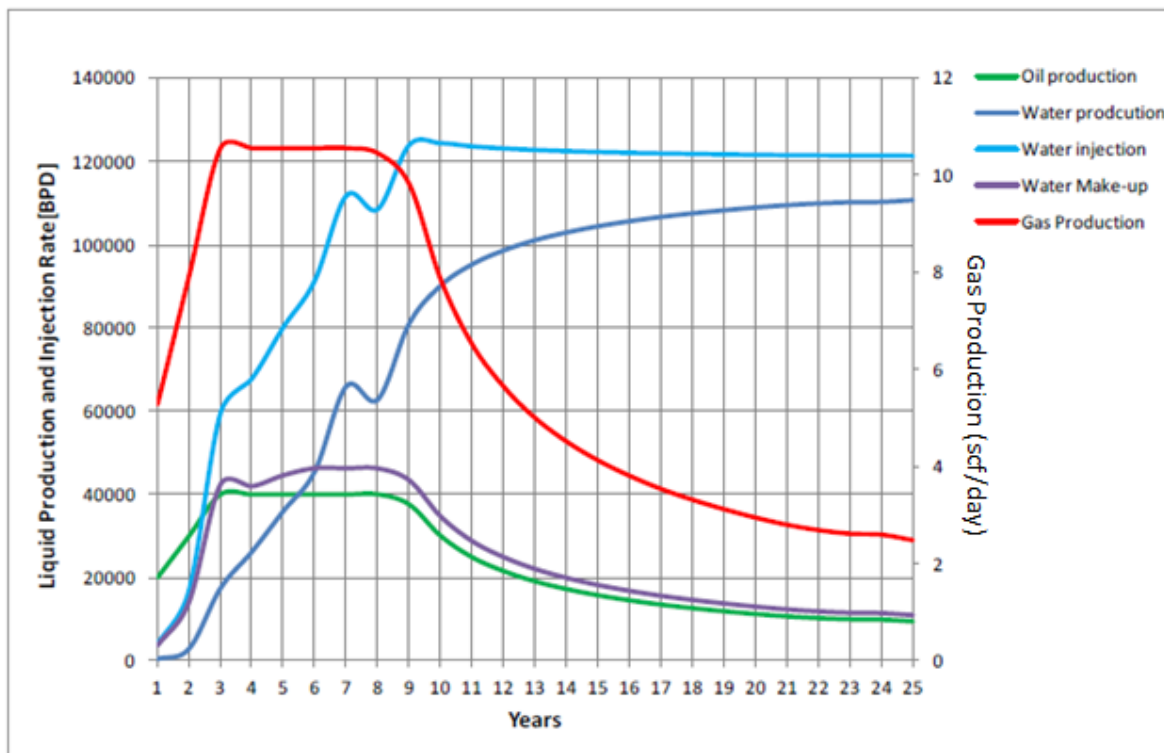
Figure 25: Production profiles for the Kingfisher oil field.
