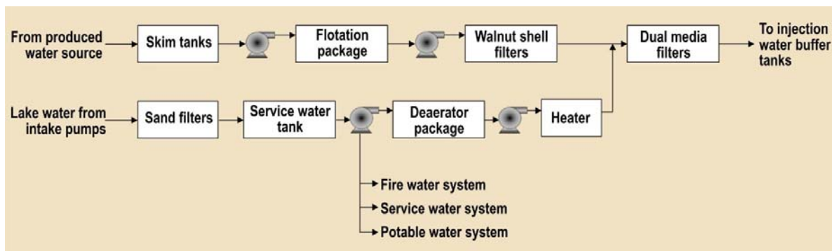
Figure 25: Produced water injection (including make-up water)
