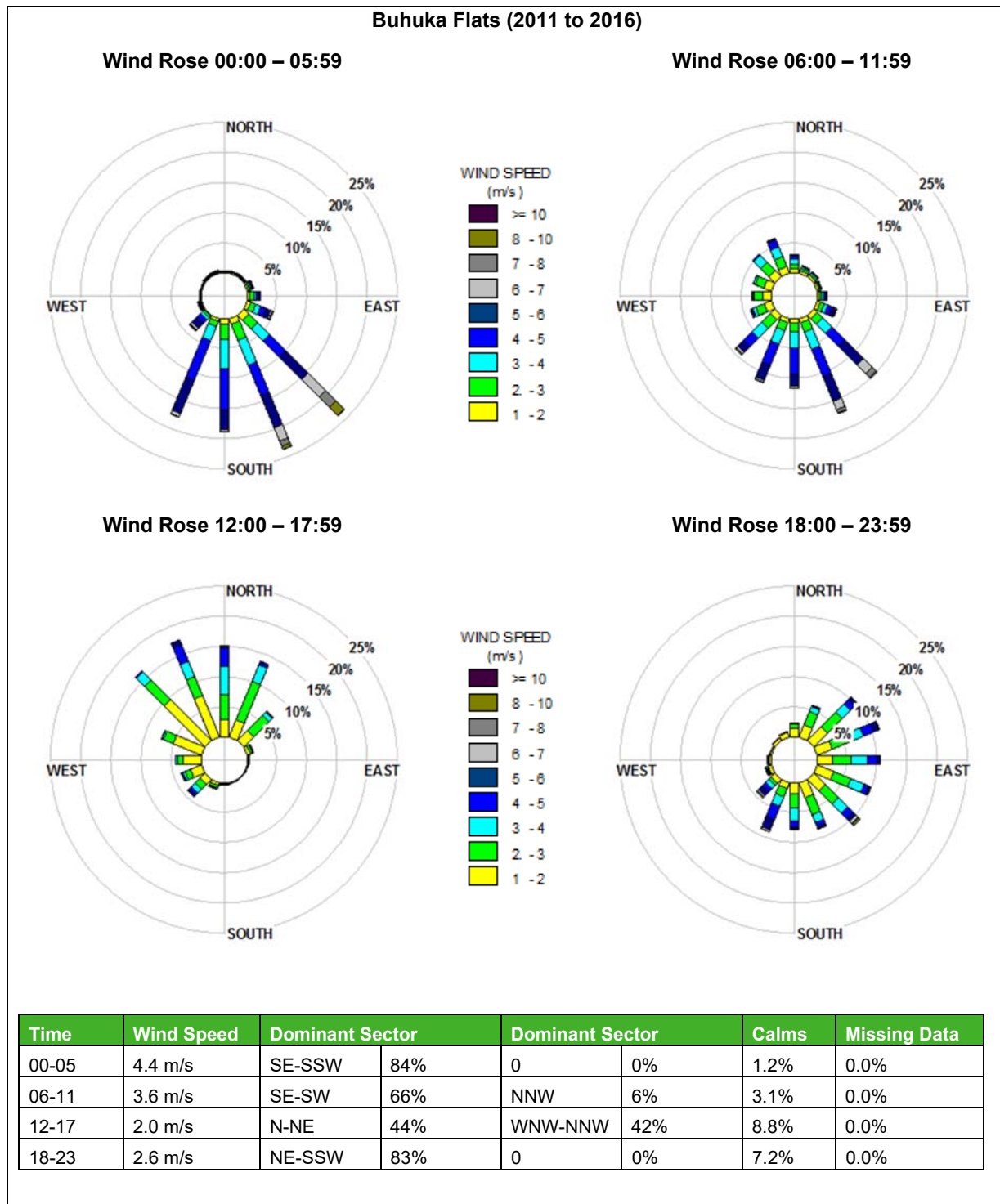
Figure 21: Diurnal Wind Roses – Buhuka Flats 2011 - 2016.
