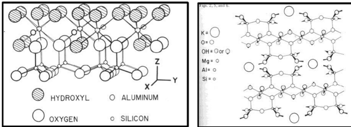
Figure 15: 1:1 (left) and 2:1 (right) clay mineral.
