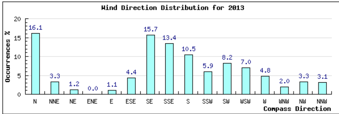
Figure 9: Buhuka Flats – Wind Direction 2013 (iWeather 2014).
