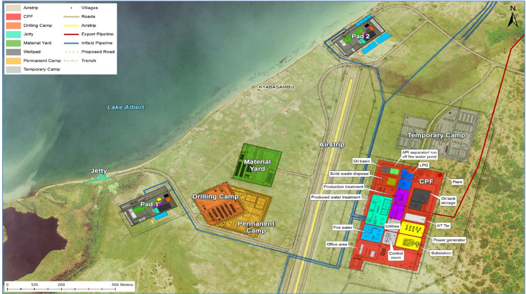
Figure 24: CPF and associated infrastructure
