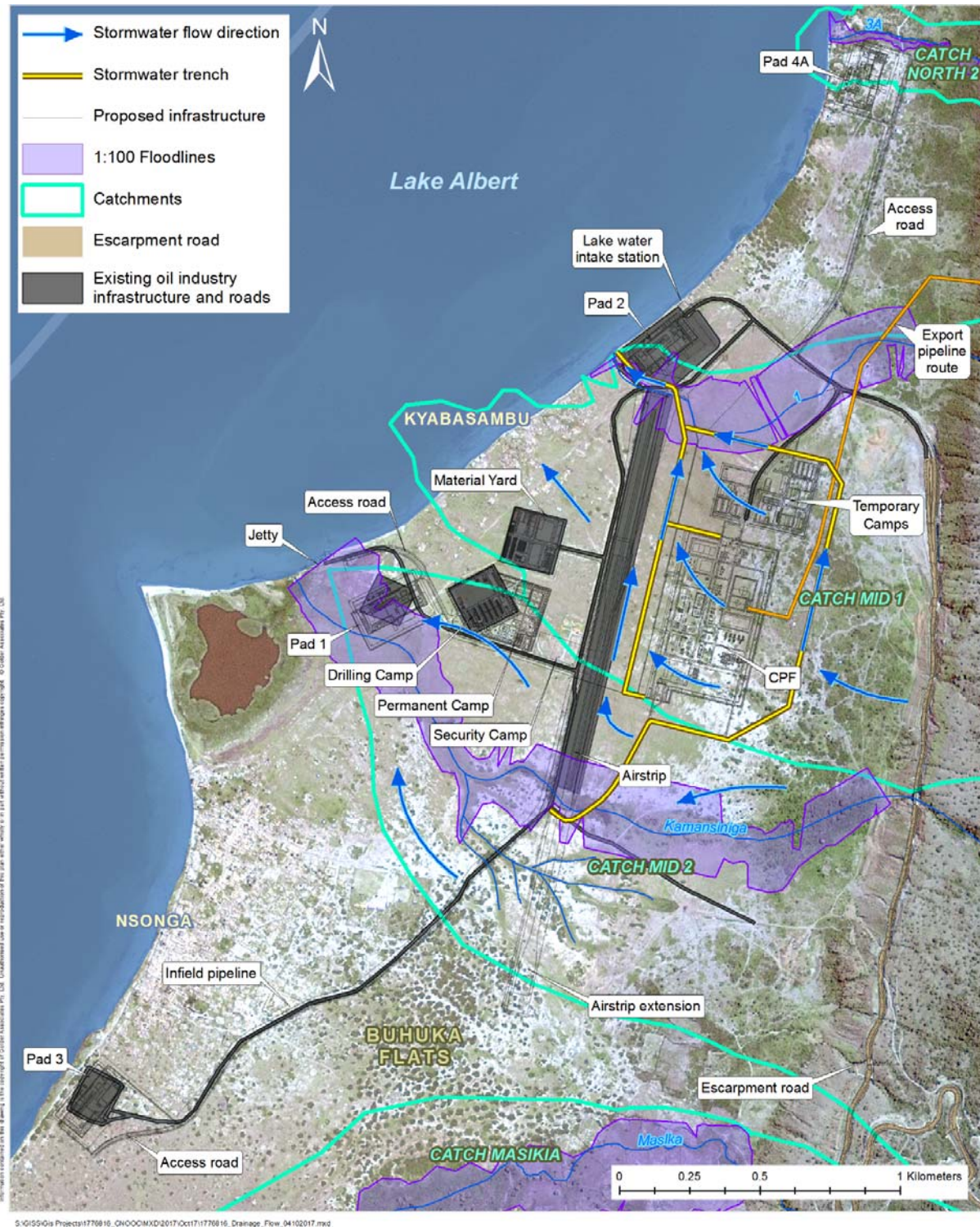
Figure 28: KDA drainage to the lake
