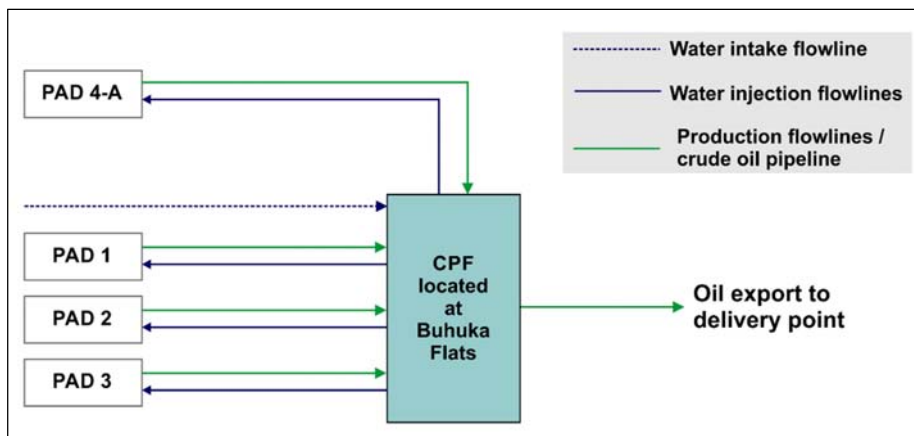
Figure 32: Schematic of production and water injection flowlines
