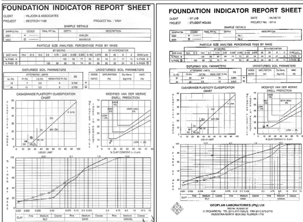
Figure 7: Typical Foundation Indicator Data for soils containing 1:1 (left) and 2:1 (right) clay mineralogy
