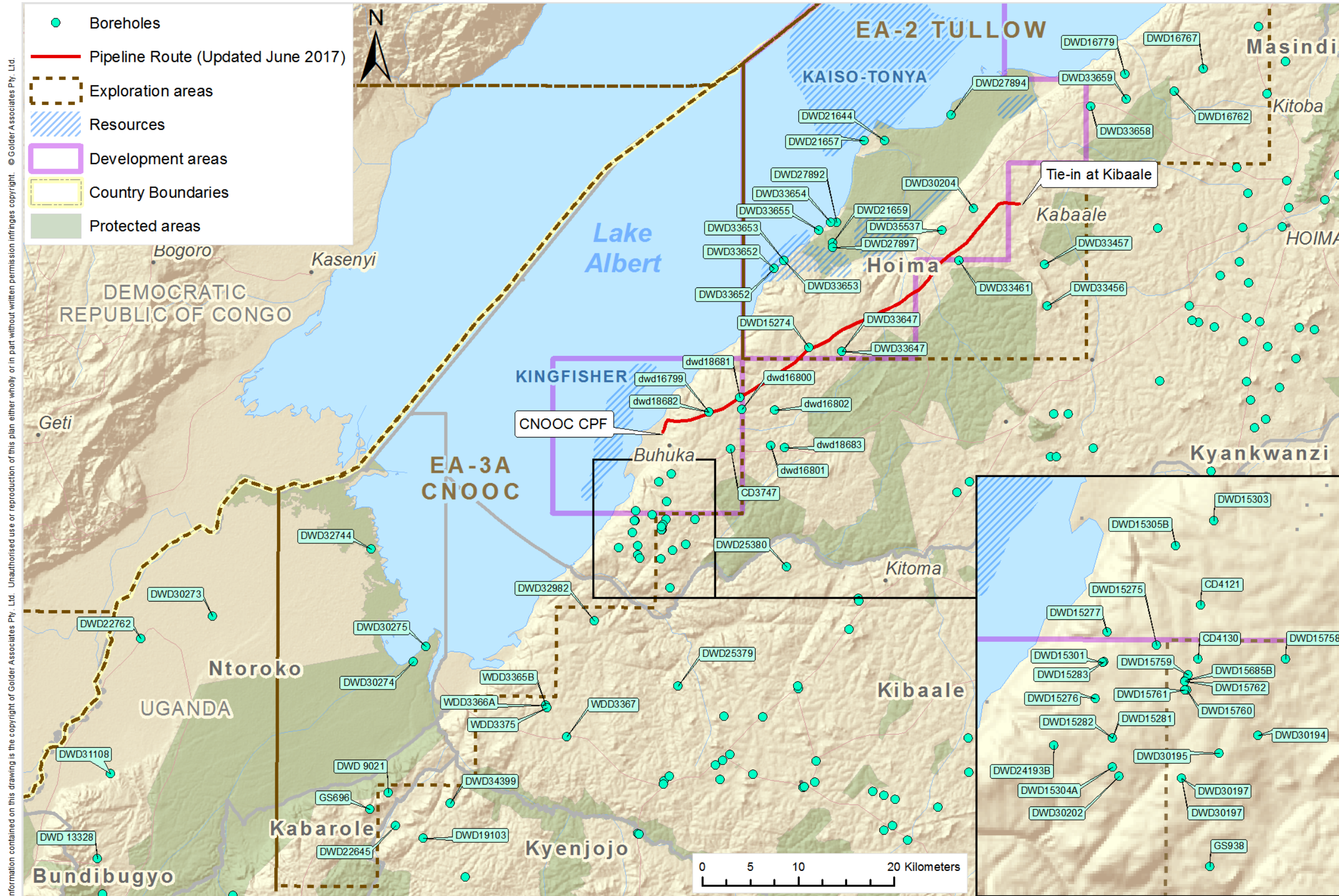
S:\GISS\GIS Projects\1776816 CNOOC\MXD\2017\Sep17\1776816 Block3A BH 20092017.mxd Figure 2: Distribution of data points – well/boreholes locations, Golder (2013) Groundwater Baseline Report for Kingfisher Block 3A
