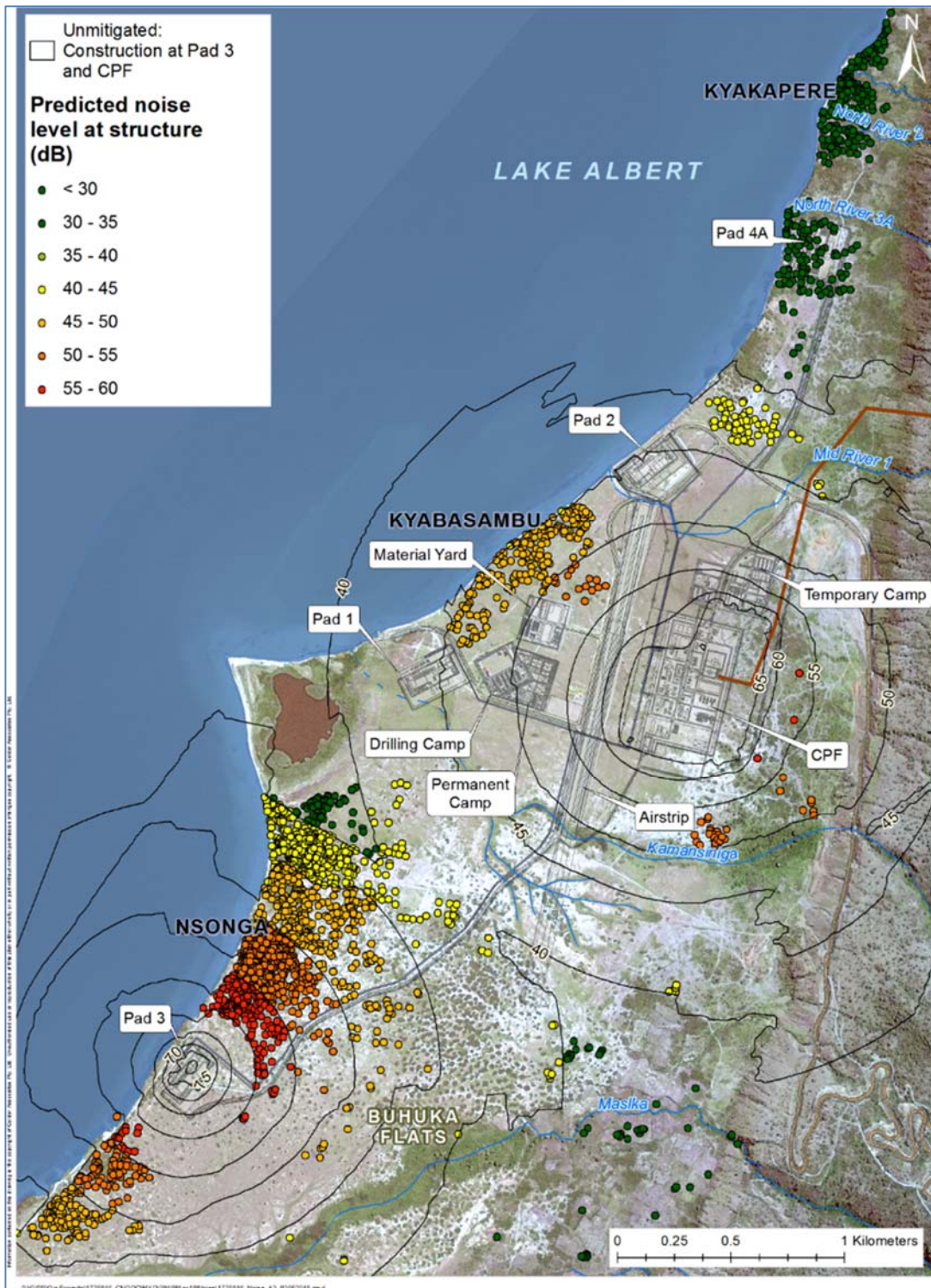
Figure 25: Example of unmitigated civil construction noise showing CPF construction and civil works ongoing simultaneously on Well Pad 3
