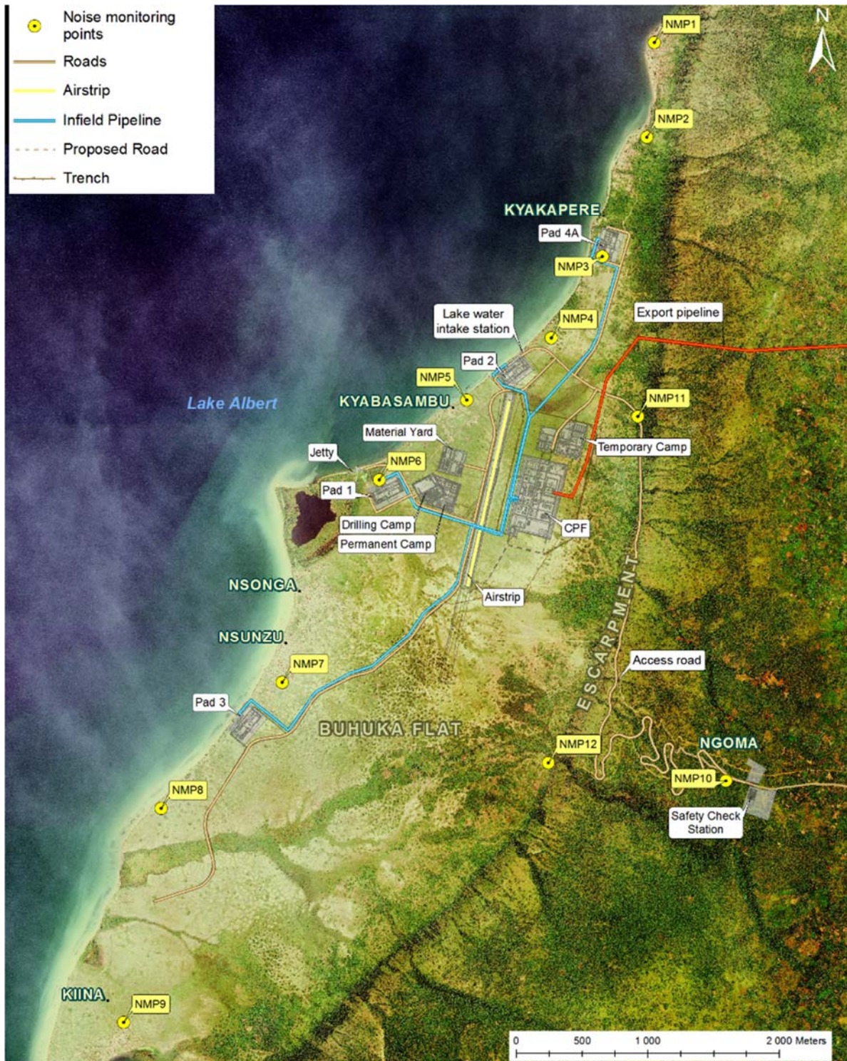
Figure 4: Local study area and baseline noise monitoring locations
