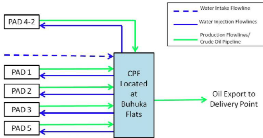
Figure 29: Flowlines schematics.
