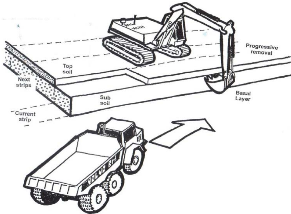
Figure 23: Removal of topsoil from a strip.
