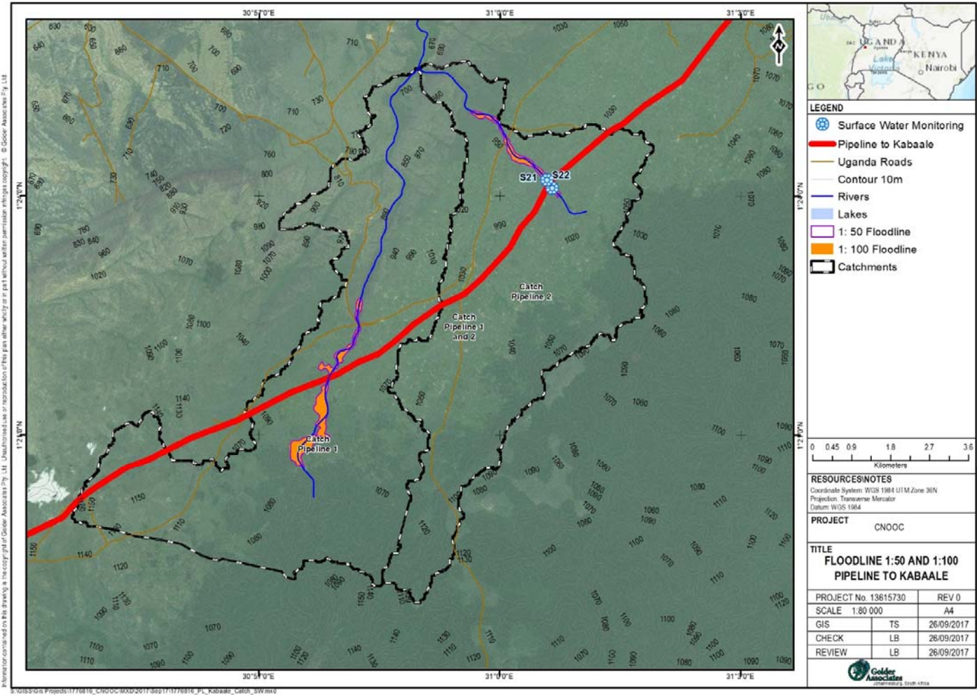
Figure 22: 1:100 floodlines along the pipeline routing
