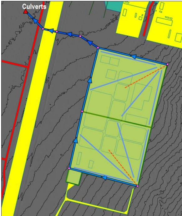
Figure 29: Northern drainage
