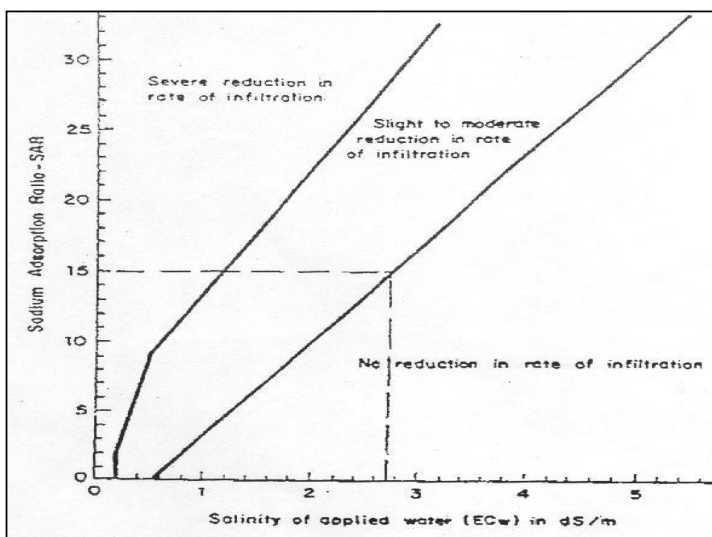
Figure 9: SAR relative to EC
