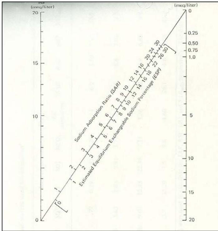
Figure 10: SAR relative to ESP
