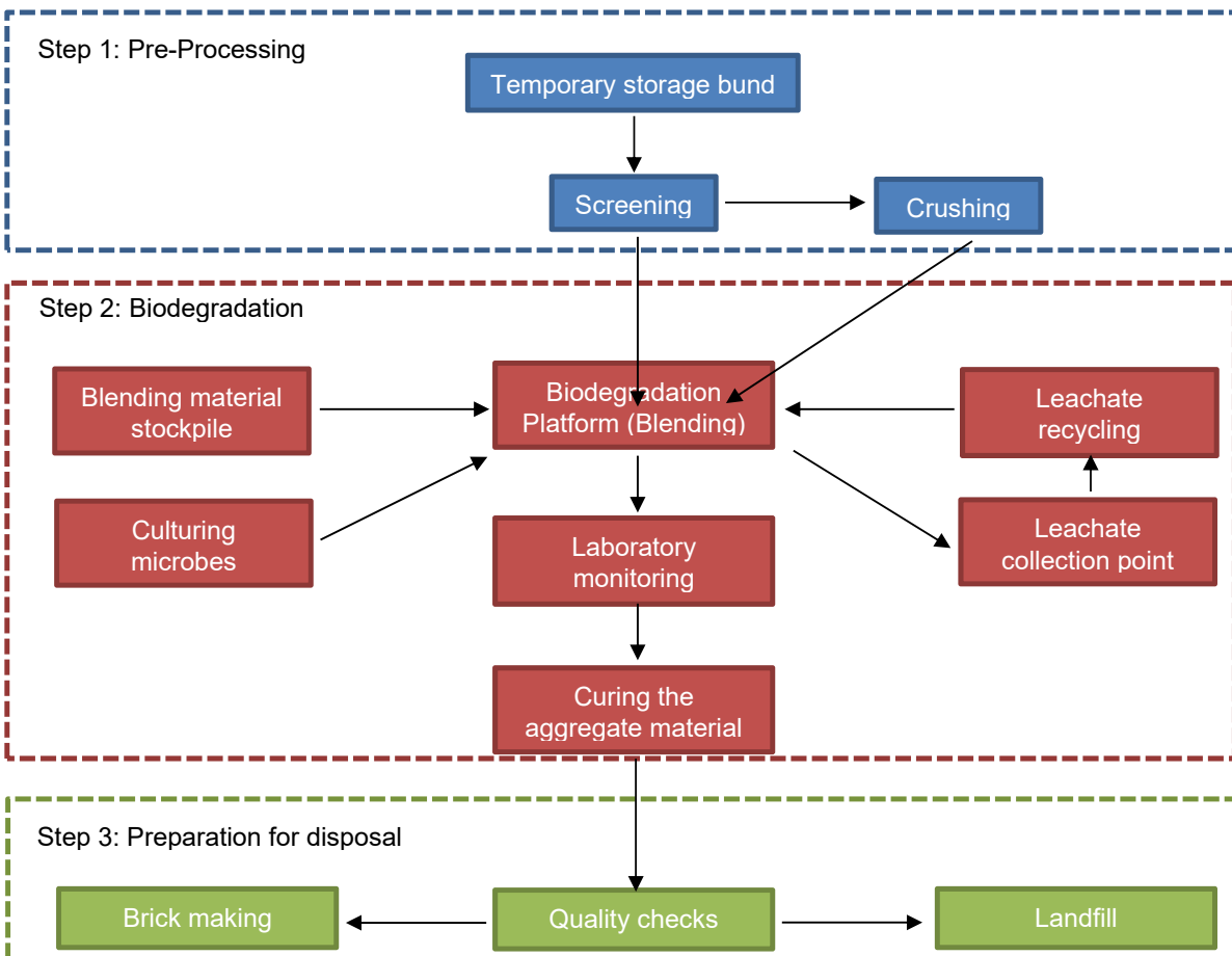
Figure 7: Flowchart of the Biodegradation Process
