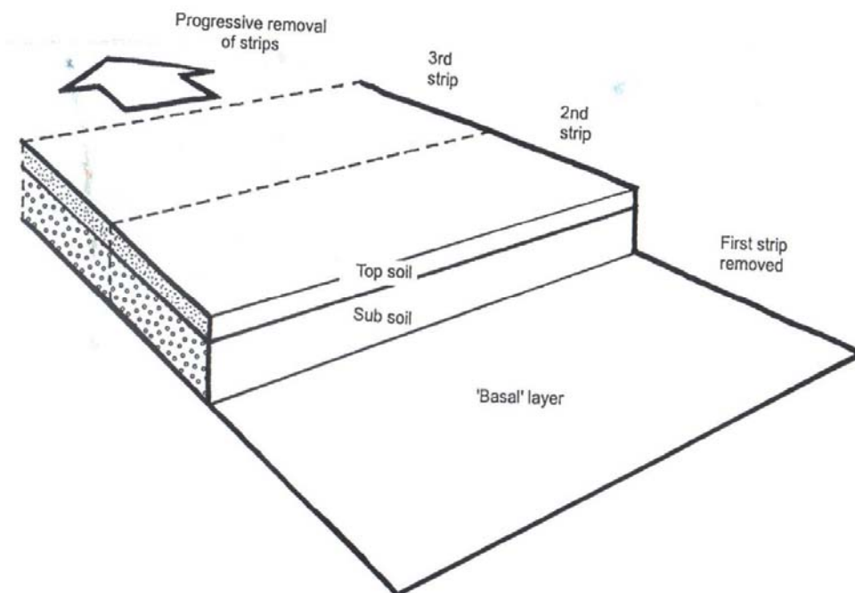
Figure 22: The bed strip system.
